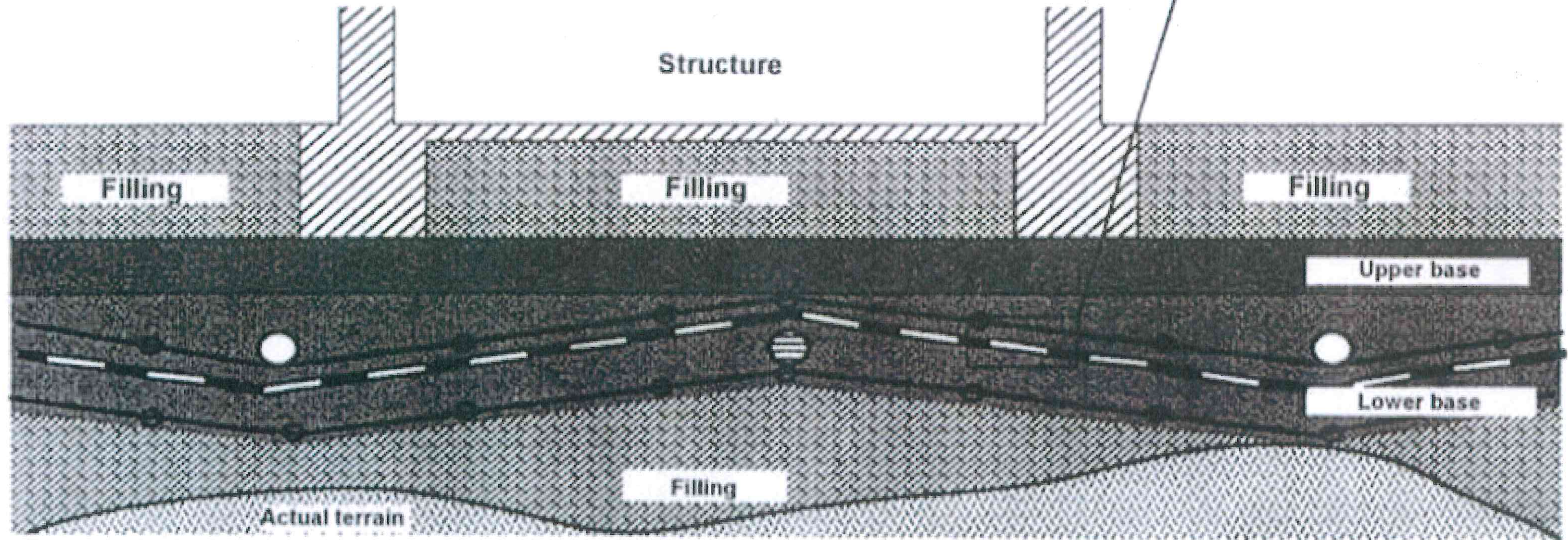
Schematic depiction of the DMT-GEOsafe-System (45)
